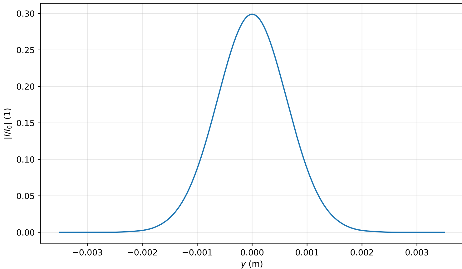
Intensity profile I(x = 0, y, z = 3.264)/I_0 , P_{in}=0.1P_{cr} , artificial time
